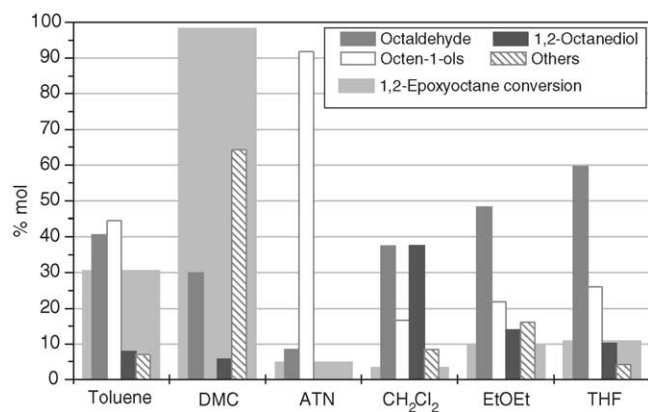
Fig. 2. 1,2-Epoxyoctane rearrangement over Al-MCM-41. Reaction conditions: catalyst loading, 40 mg; temperature, 120 °C and time, 2 h. DMC: dimethylcarbonate; ATN: acetonitrile; CH 2 Cl 2 : dichloromethane; EtOEt: diethylether; THF: tetrahydrofuran; Others including: 2-Octanone; 1,4-epoxyoctane; 2-oct-2-enyloxy-octan-1-ol; glycoethers and 2-methoxyoctyl 1-(methoxymethyl)heptyl carbonate.
