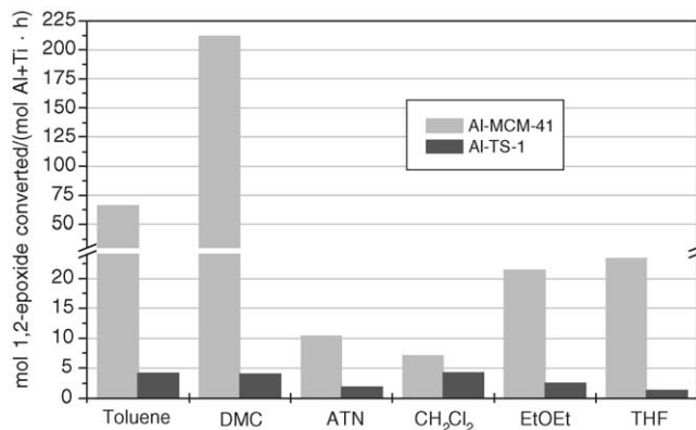
Fig. 5. Turnover frequency in 1,2-epoxyoctane isomerization over Al-MCM-41 and Al-TS-1 catalysts.
