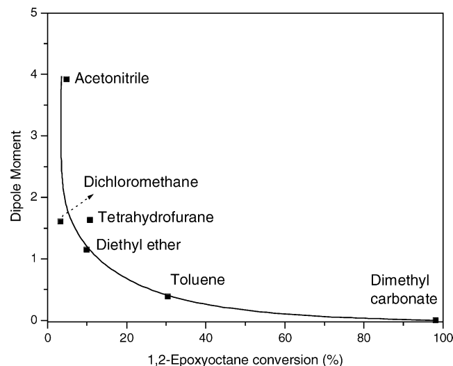
Fig. 4. 1,2-Epoxyoctane conversion over Al-MCM-41 as a function of the polarity of solvents.
