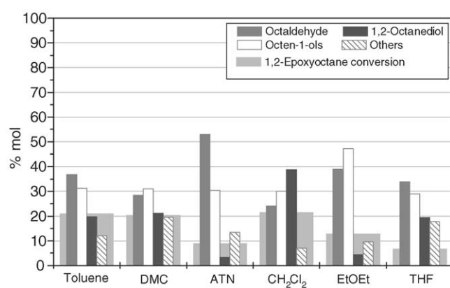
Fig. 3. 1,2-Epoxyoctane rearrangement over Al-TS-1. Reaction conditions: catalyst loading, 400 mg; temperature, 120 °C; time, 3 h. DMC: dimethylcarbonate; ATN: acetonitrile; CH 2 Cl 2 : dichloromethane; EtOEt: diethylether; THF: tetrahydrofuran; Others including: 2-Octanone; 1,4-epoxyoctane; 2-oct-2-enyloxy-octan-1-ol; glycoethers and 2-methoxyoctyl 1-(methoxymethyl)heptyl carbonate.
