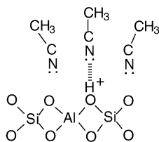
Scheme 4. Neutralization of acid sites by acetonitrile.
