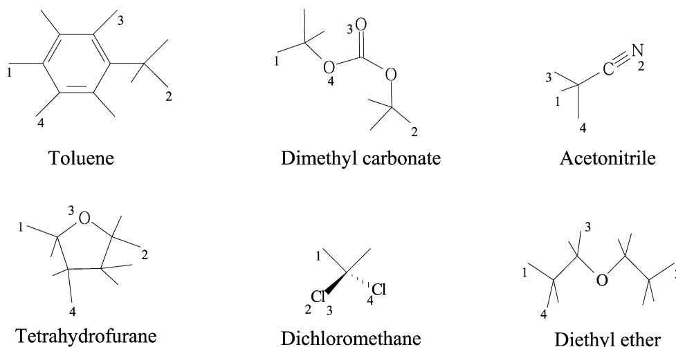
Scheme 1. Structural formulas and numbering of atoms for solvent molecules.
