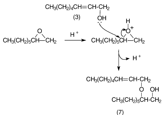
Scheme 3. Nucleophilic attack of octenols to the epoxide: (7) 2-oct-2-enyloxy-octan-1-ol.
