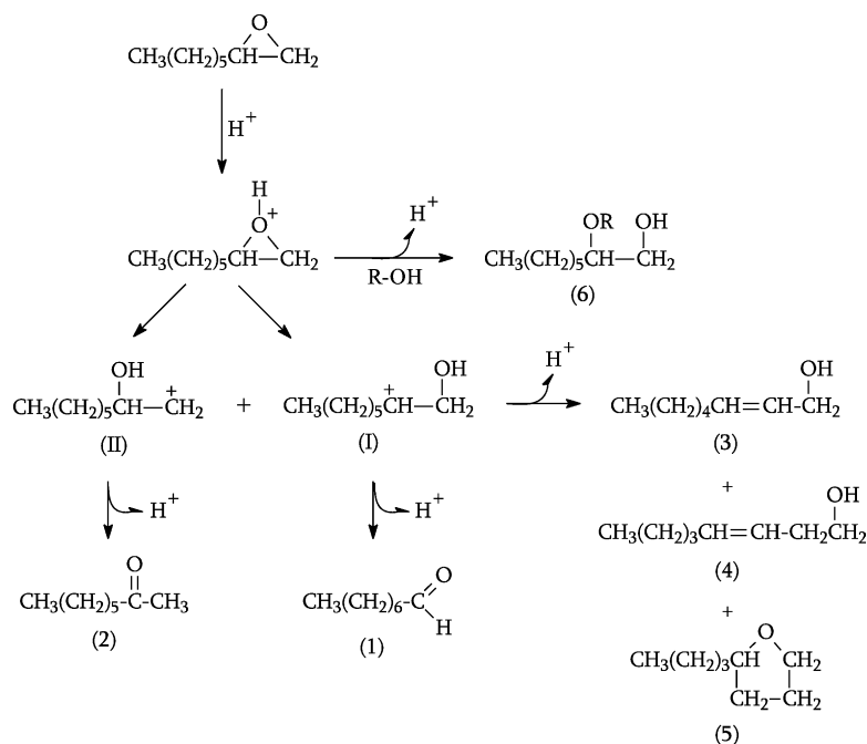
Scheme 2. Acid catalyzed mechanism of the isomerization of 1,2-epoxyoctane: (1) Octaldehyde; (2) 2-Octanone; (3) 2-octen-1-ol; (4) 3-octen-1-ol; (5) 1,4-epoxyoctane and (6) 1,2-glycolethers.
