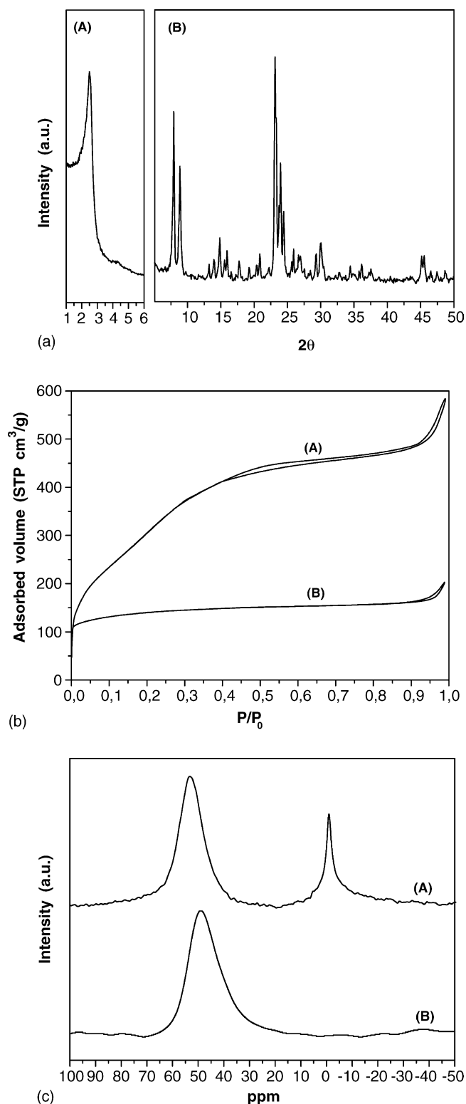
Fig. 1. Characterization results of Al-MCM-41 (A) and Al-TS-1 (B). (a) XRD (b) N 2 adsorption isotherms (c) 27 Al-MAS-NMR.
