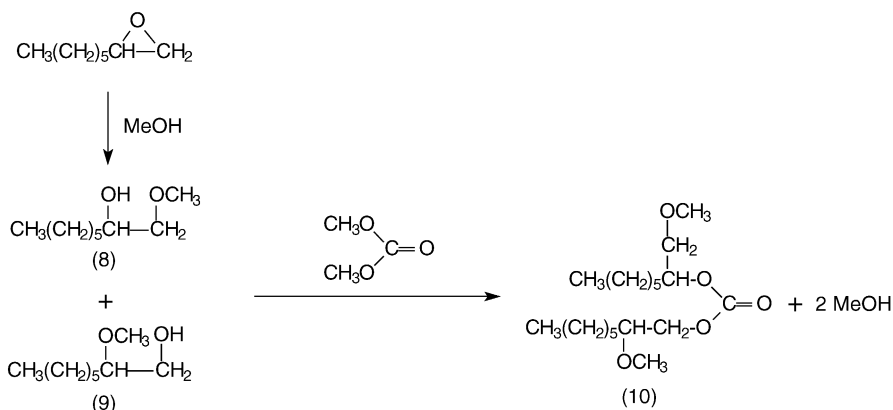
Scheme 5. Formation mechanism of glycolethers (8) and (9) and 2-methoxyoctyl-(methoxymethyl)heptyl carbonate (10) using dimethyl carbonate as solvent.
